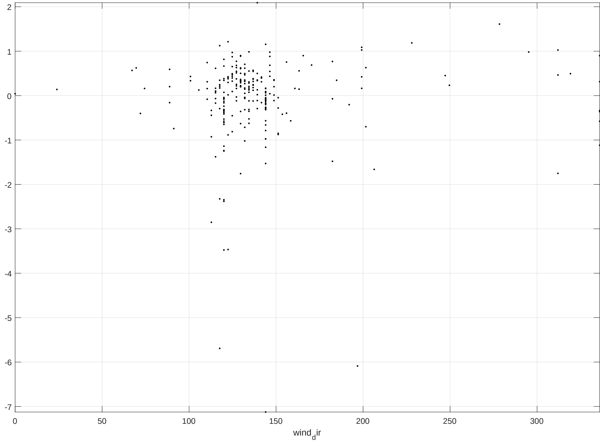
rel h um|temp: Residuals on wind d ir
